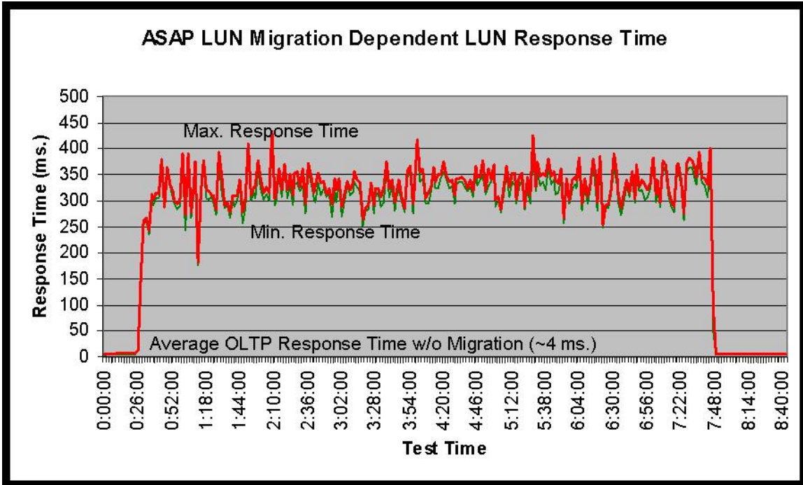
Figure 10. ASAP LUN migration dependent LUN response time
