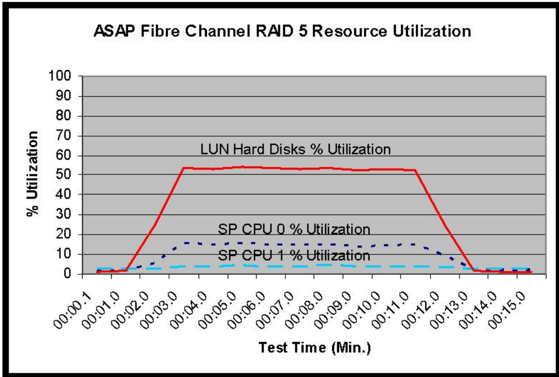
Figure 4. ASAP rebuild for a Fibre Channel RAID 5 group LUN
