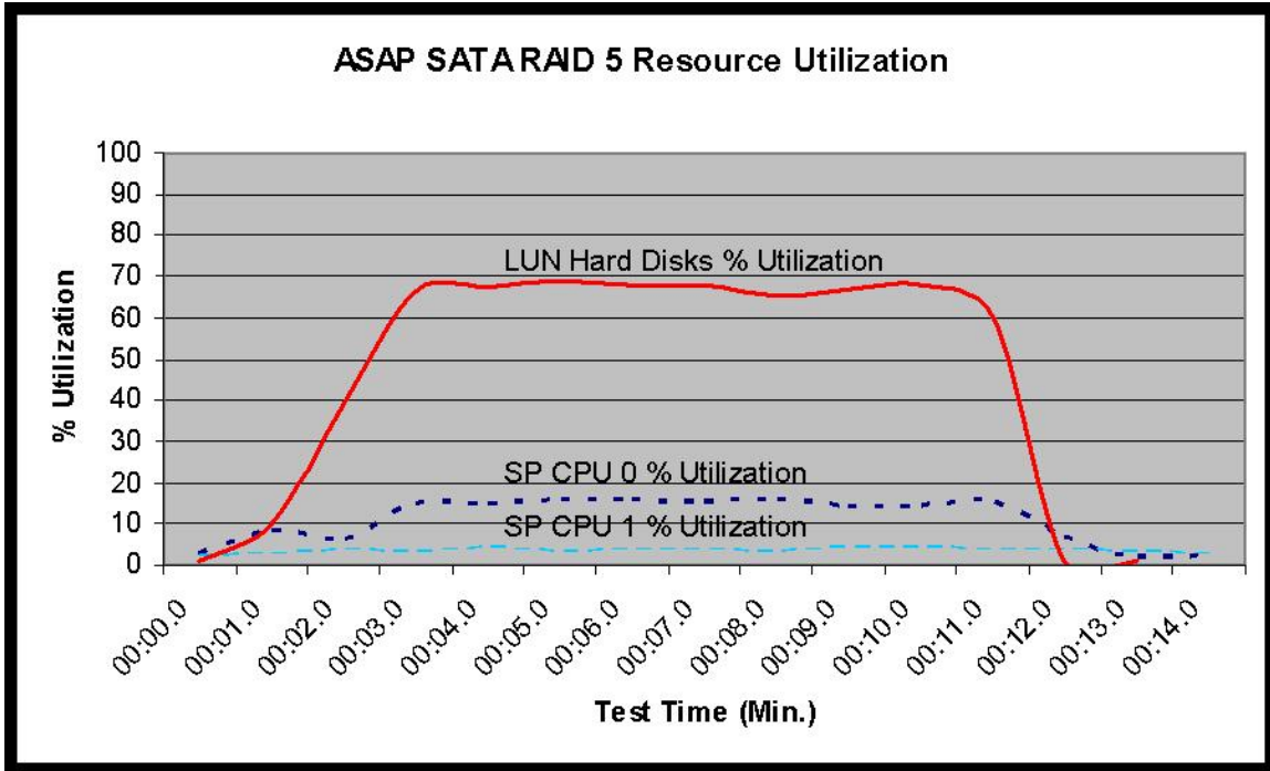
Figure 3. ASAP rebuild for a SATA RAID 5 group LUN
