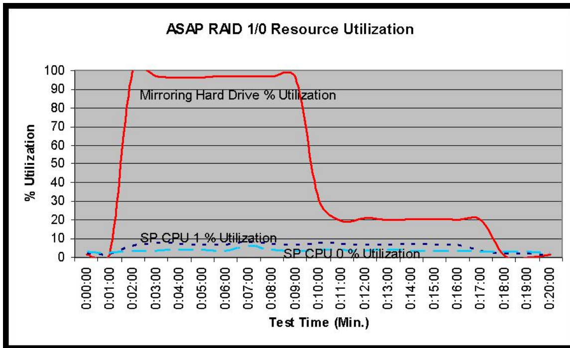
Figure 2. ASAP rebuild for a Fibre Channel RAID 1/0 group LUN
