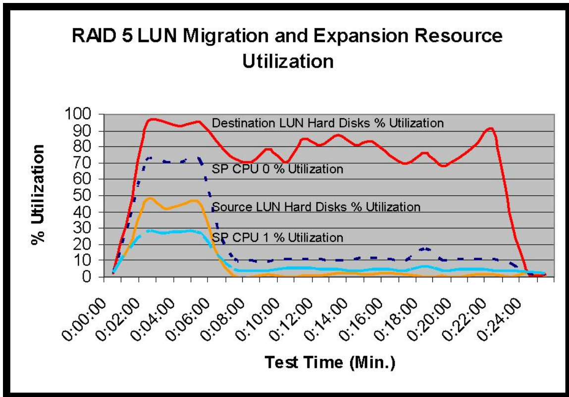
Figure 1. ASAP LUN migration resource utilization
