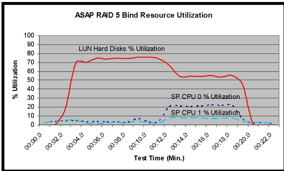
Figure 5. RAID 5 ASAP LUN bind resource utilization
