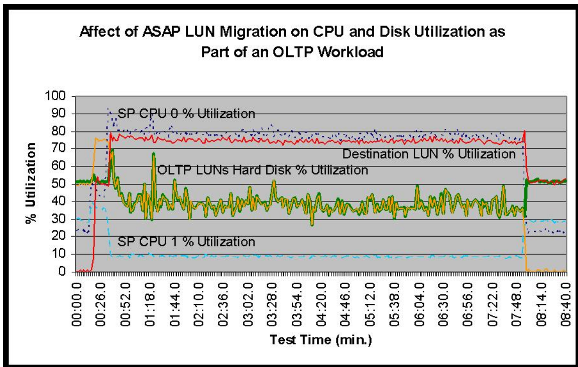
Figure 9. ASAP LUN migration resource utilization under load
